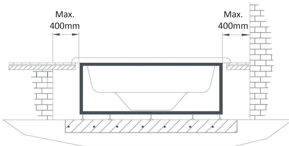
Diagram of minimum distance around the Spa
