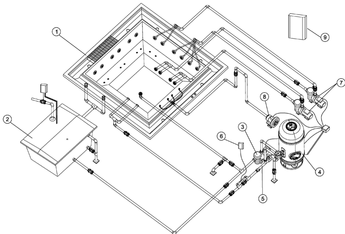
General diagram of Spa with Overflow
