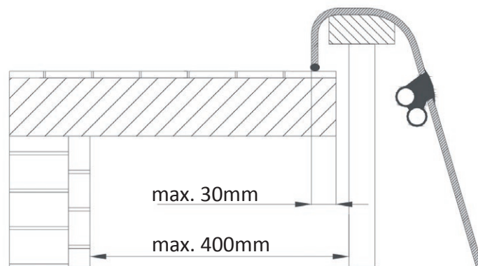
Detail of Lip Sealing
