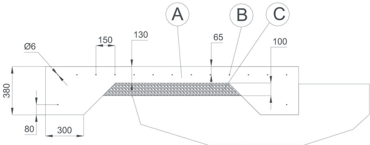
A: Concrete slab B: Steel rod C: Compacted sand All measurements in mm.
