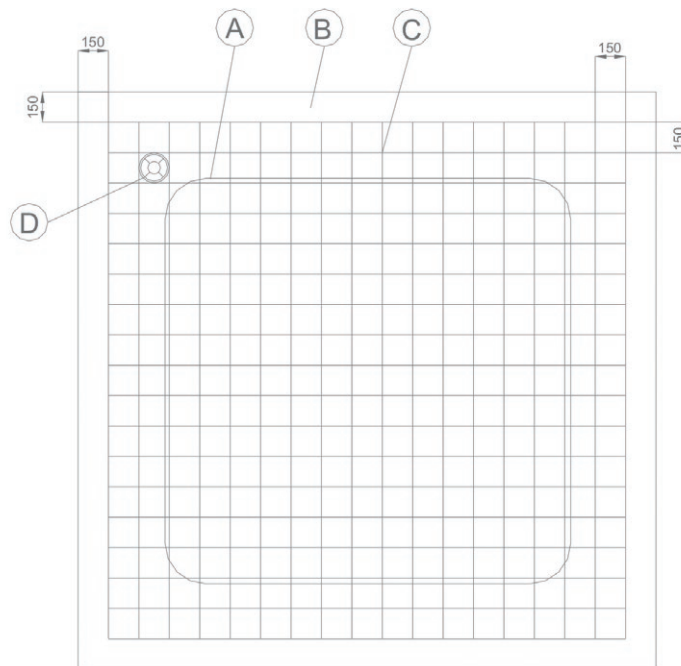
Foundations diagram
