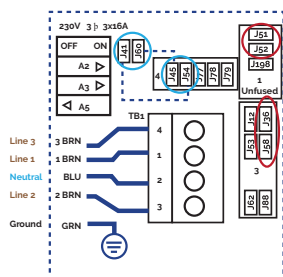
Three-phase line 400V BP013G1 & BP013G2
